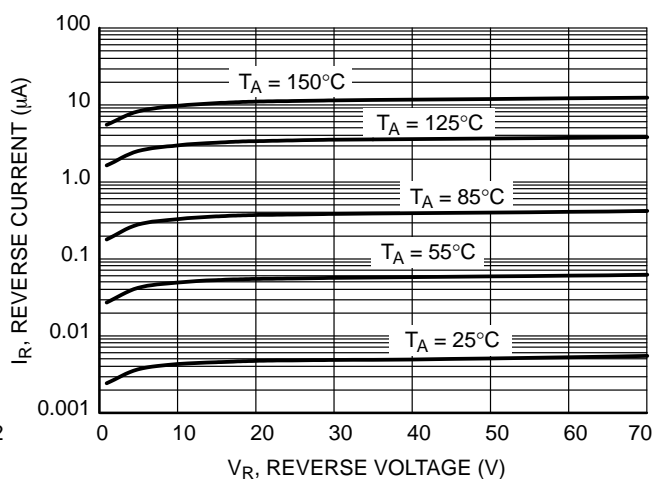
Figure 2. Leakage Current
