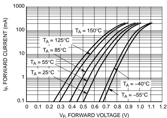
Figure 1. Forward Voltage
